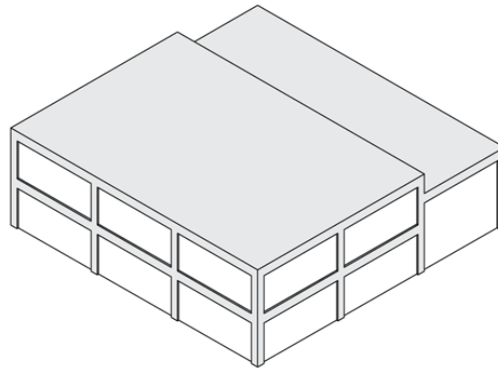
Gambar 3. 8 Ilustrasi split level Sumber : (FEMA P-154, 2015)
