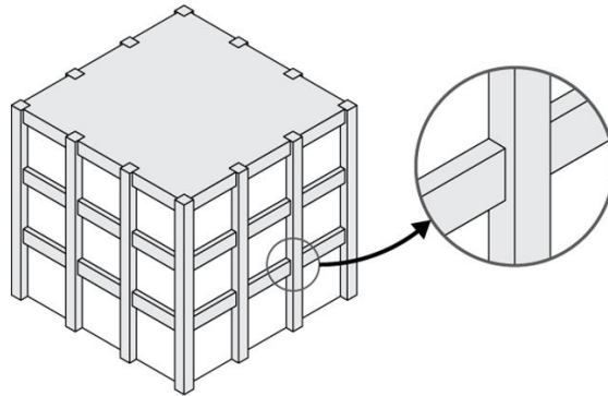
Gambar 3. 14 Ilustrasi beams do not align with coloums Sumber : (FEMA P-154, 2015)
