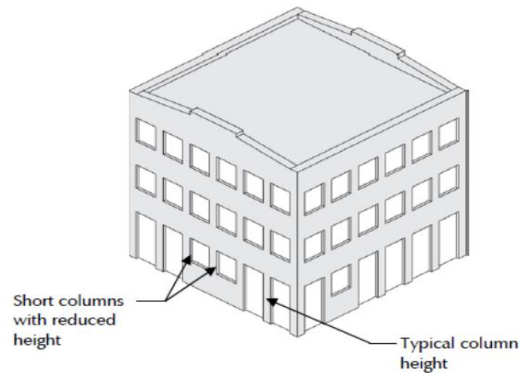
Gambar 3. 7 Ilustrasi short coloumn Sumber : (FEMA P-154, 2015)
